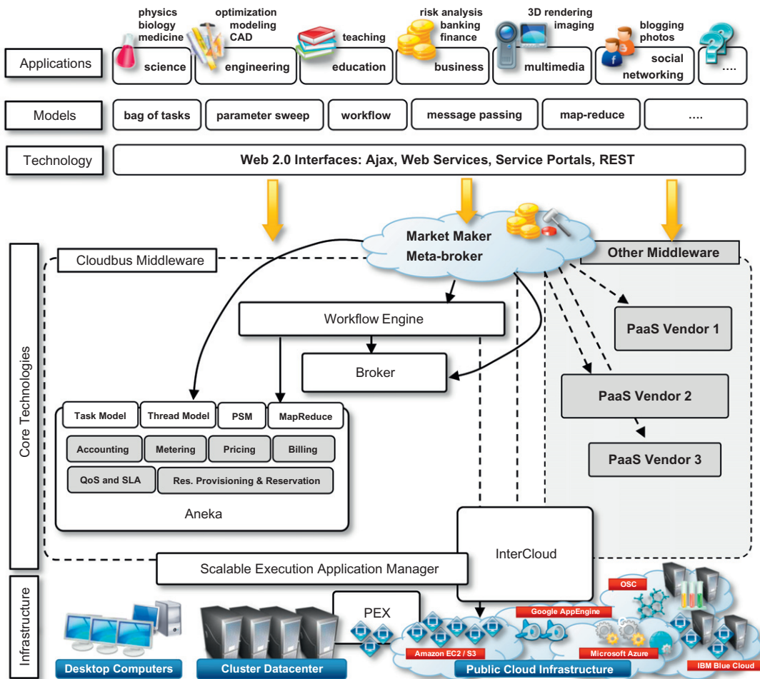
FIGURE 11.6 Cloudbus Toolkit.
