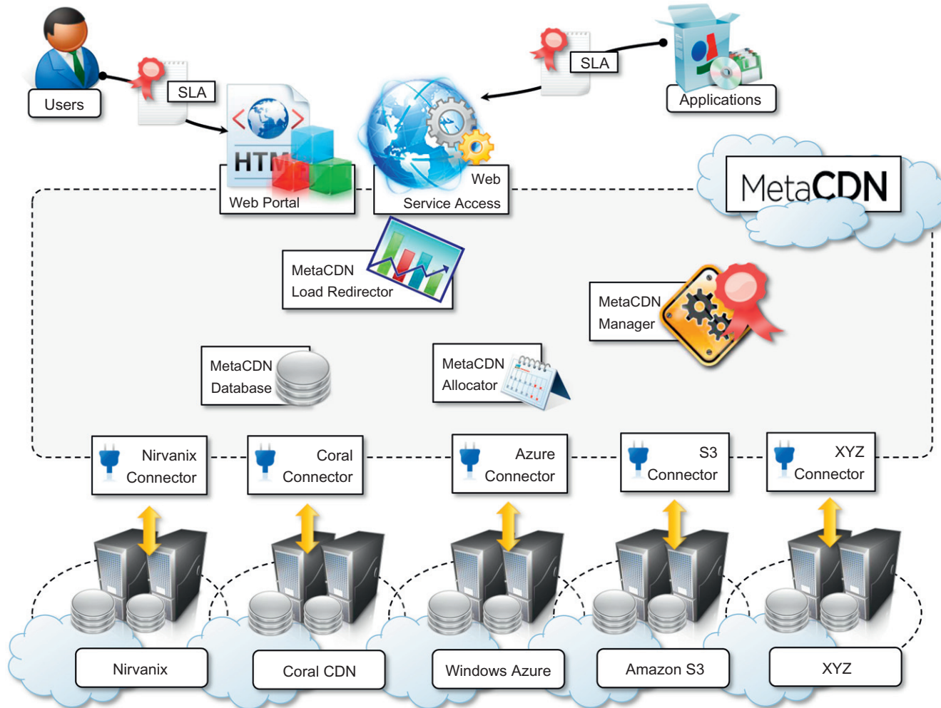
FIGURE 11.13 MetaCDN architecture.
