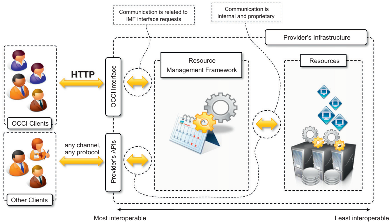
FIGURE 11.8 OCCI reference scenario.
