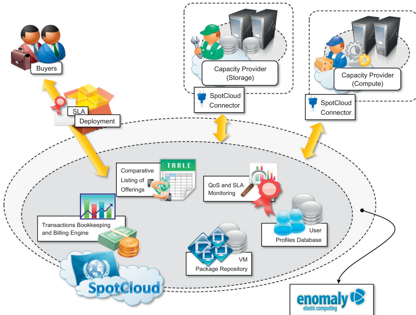
FIGURE 11.14 SpotCloud market architecture.
