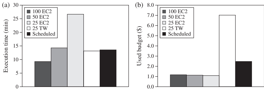
FIGURE 10.11. Experimental evaluation of medical image registration using CometCloud - Comparison of performance and costs with/without autonomic scheduling. (a) Execution time varying the number of nodes of EC2 and TW. (b) Used budget over time varying the number of nodes for EC2 and TW.
