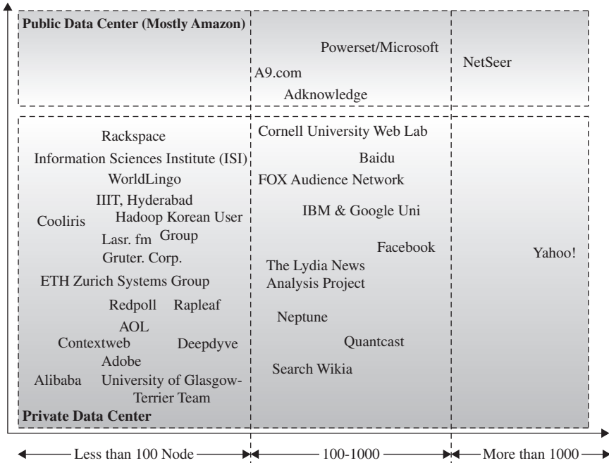
FIGURE 14.4. Organizations using Hadoop to run distributed applications, along with their cluster scale.
